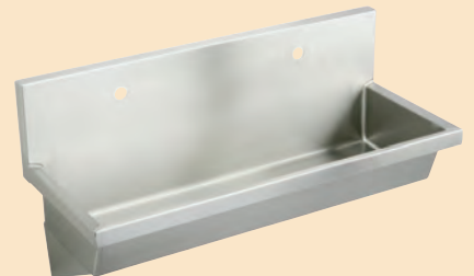
EWMA48202 Multiple station wash sink with 10" high backsplash.
